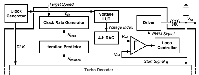
Fig. 8. The developed DVFS scheme including a throughput prediction engine and a DC-DC converter.
