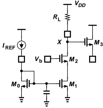
Fig. 16. Arrangement for measuring device noise.
