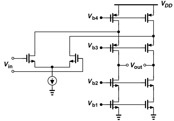
Fig. 11. Folded-cascode op amp (common-mode feedback not shown).
