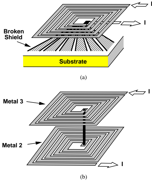
Fig. 18. (a) Inductor with broken shield, (b) stacked inductors.
