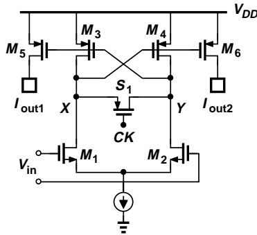
Fig. 10. Simple comparator for measuring metastability.
