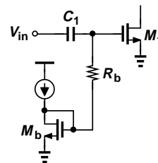
Fig. 8. Bias circuit using n-well resistor.
