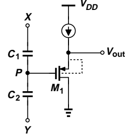
Fig. 15. Capacitor mismatch measurement.
