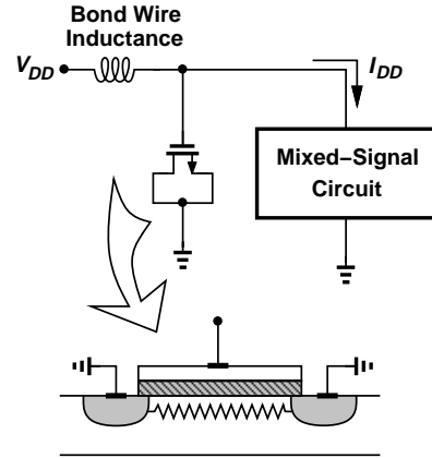
Fig. 6. MOS capacitors as by-pass elements along with illustration of channel resistance.
