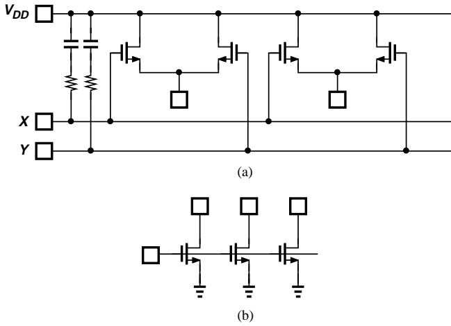
Fig. 13. Structures for measuring device mismatch.
