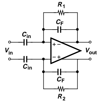
Fig. 12. Arrangement for measuring op amp distortion.
