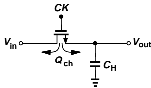
Fig. 4. Input-dependent charge injection.
