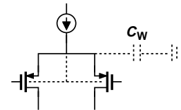
Fig. 7. N-well capacitance in a PMOS differential pair.
