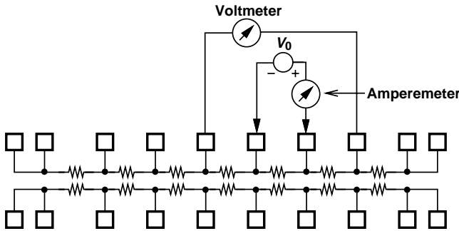
Fig. 14. Topology for measuring resistor mismatch.
