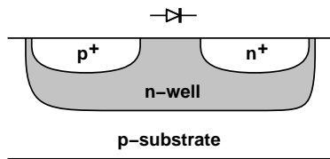
Fig. 20. Floating varactor in CMOS technology.
