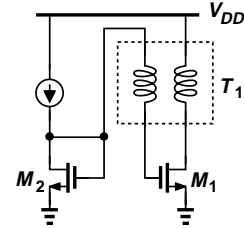
Fig. 21. Transformer-based oscillator.
