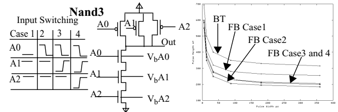
Figure 4. Series Stack Nand3
