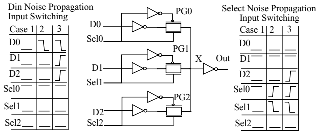
Figure 8. Three Input Mux
