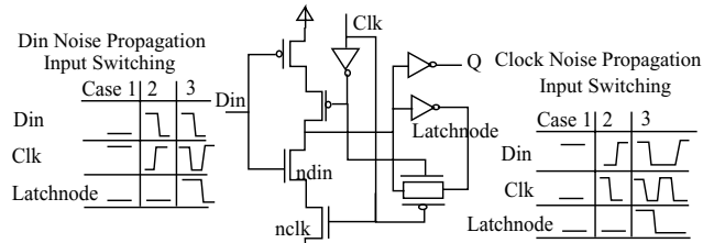
Figure 11. Latch Circuit
