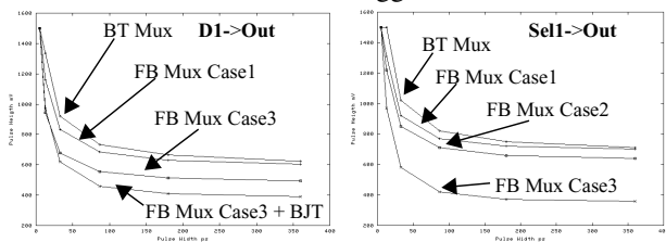
Figure 9. Mux Propagated Noise Curves
