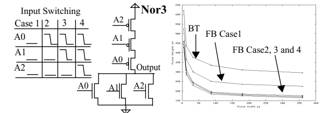
Figure 5. Parallel Stack Nor3
