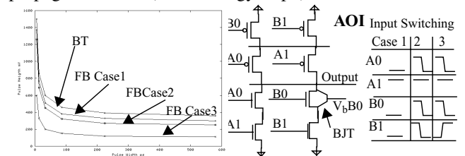
Figure 6. Parallel and Series Stack AOI
