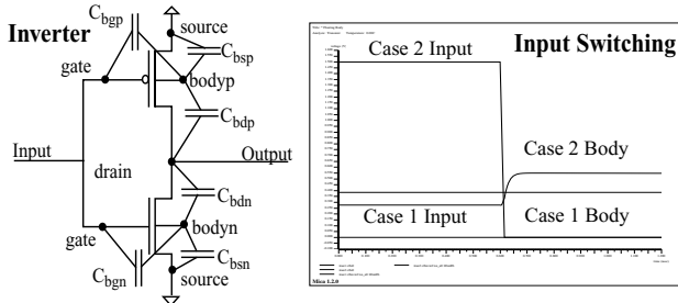
Figure 2. Inverter Input Switching
