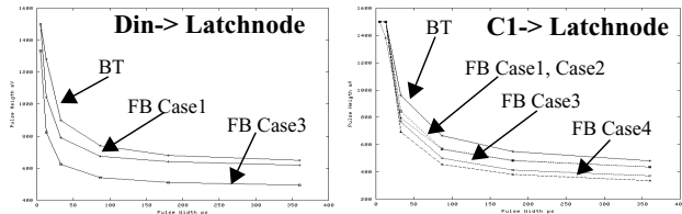
Figure 12. Latch Propagated Noise Curves
