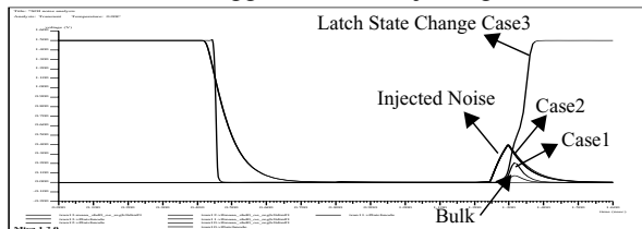
Figure 14. Latch Failure Spice Simulations
