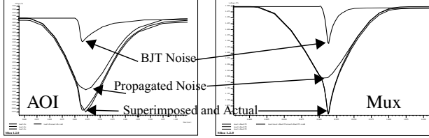
Figure 7. AOI and Mux BJT N
