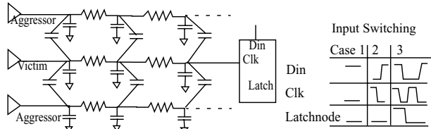
Figure 13. Spice Setup for Switching History
